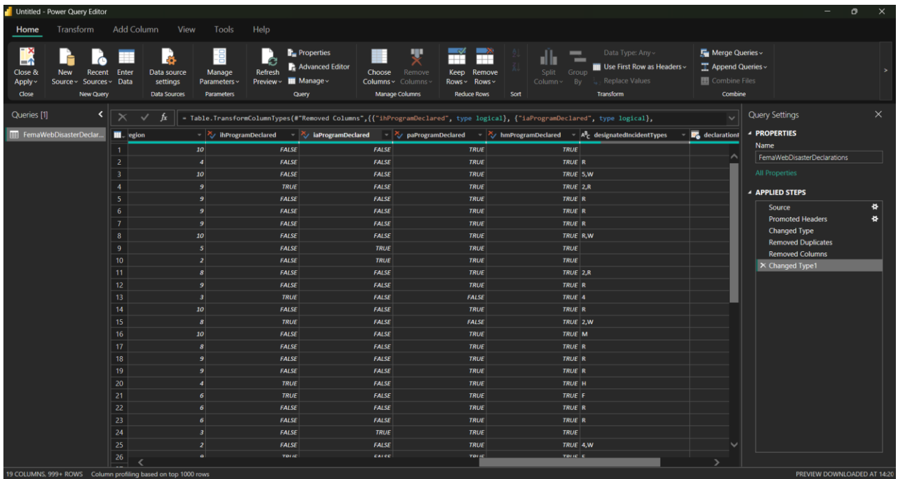
Fig 1.4 Changed Datatype
